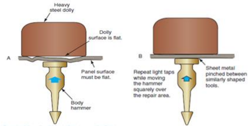
Figure 2- 29 Using light hammer blows from the front to remove the damage
