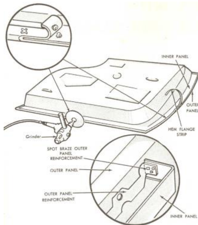
Figure 2- 45 Removing hem flange of door, prior to replacing the outer panel.
