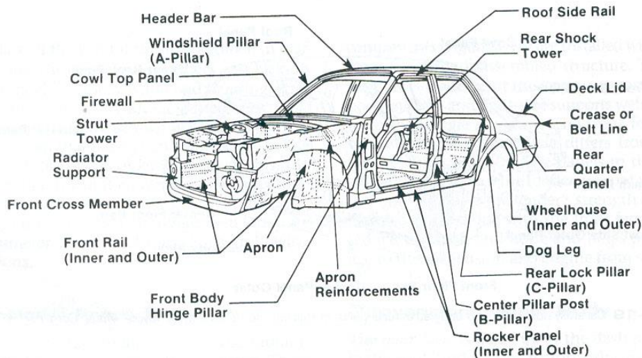
Figure1- 2 Body Constructions
