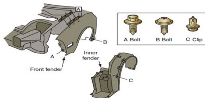
Figure 2- 13 removal fender
