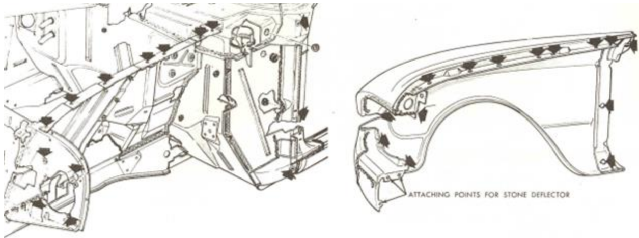
Figure 2- 38 Attaching point of fender and stone deflector
